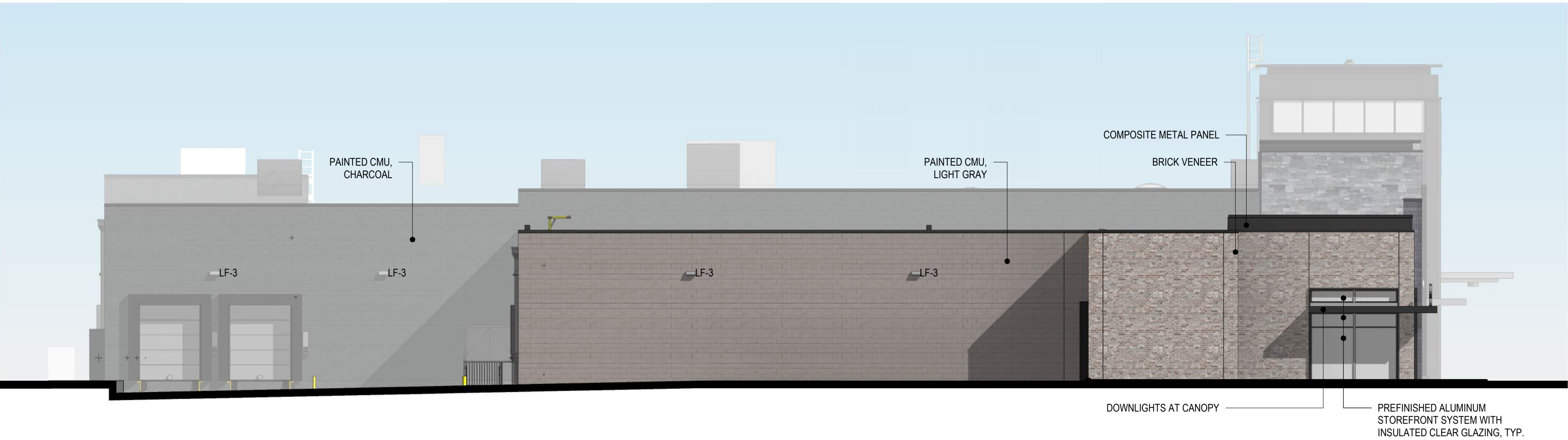
WEST (SIDE) ELEVATION
