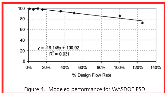
CDS Unit Performance for Ecology PSD d 50 = 125 μm
